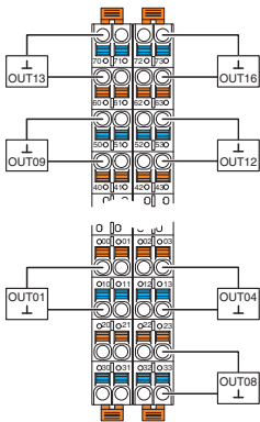
Connection in 2-conductor technology
